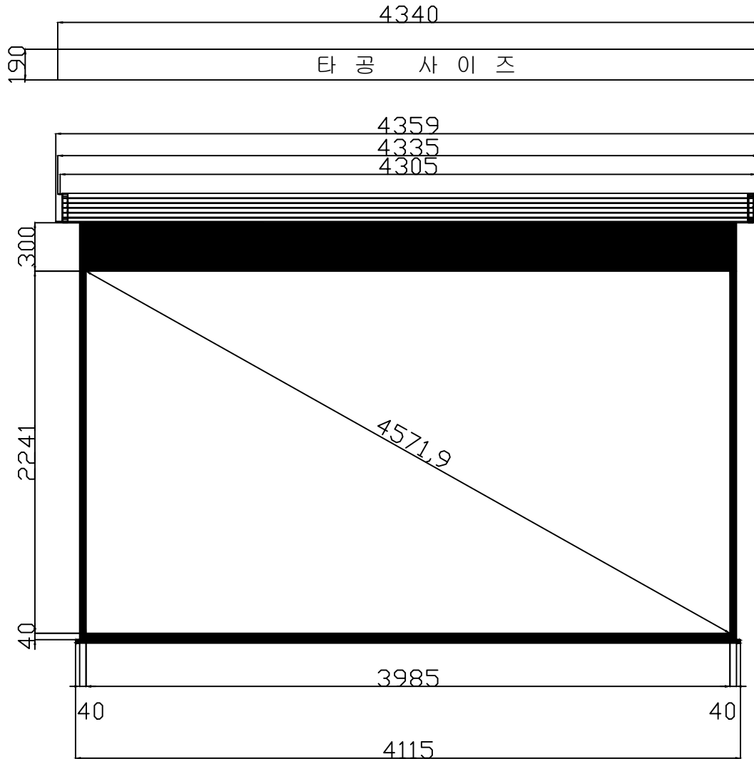
Front View
